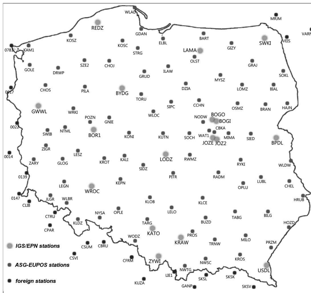
Fig. 1 ASG-EUPOS network.
