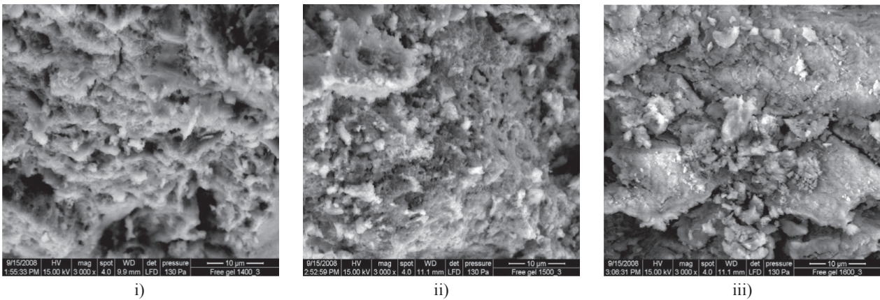
Figure 2a. Scanning Electron Micrograph of the sintered gel samples (no additive) (i): sintered at 1400^\circ\text{C} (ii) sintered at 1500^\circ\text{C} (iii) sintered at 1600^\circ\text{C} .
